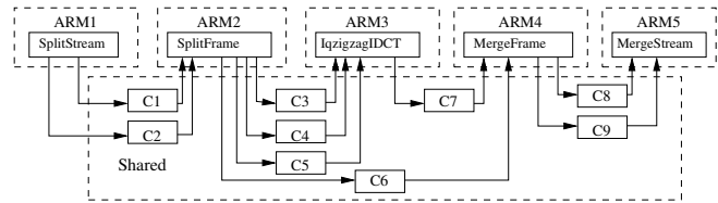
Figure 14. MJPEG Decoder application and a mapping
