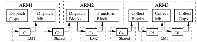
Figure 16. MPEG-2 Decoder application and a mapping
